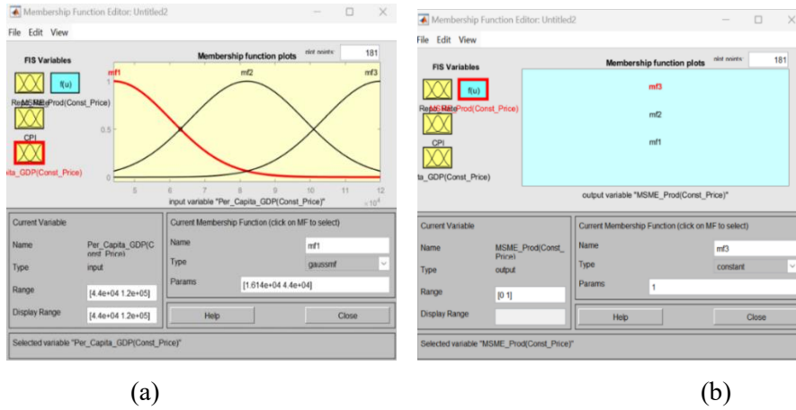
Fig. 4. (a) Gaussian Membership function for Input variable Per Capita GDP (Constant Price); (b) Output Variable MSME Prod (Constant Price)
