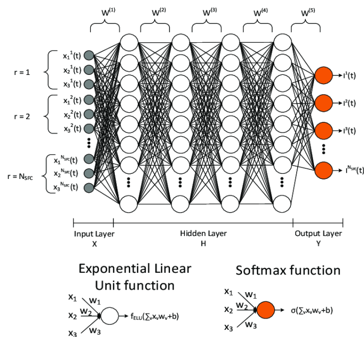
Fig. 1. GPT-4 Architecture
